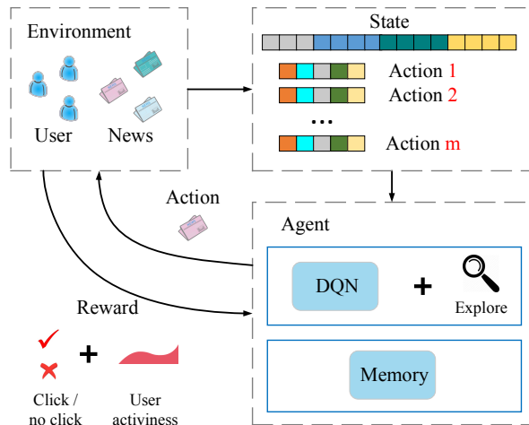
Figure 2: Deep Reinforcement Recommendation System
