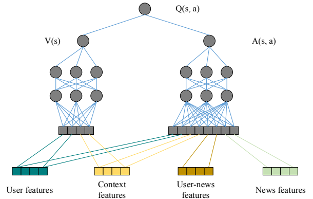
Figure 4: Q network
