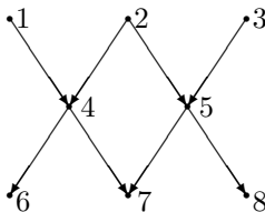
FIG. 4.1. Hasse diagram of the poset P in Example 4.7.
